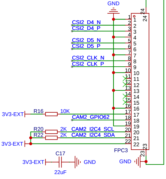
CAMERA2 (CSI2)
