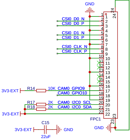
CAMERA0 (CSI0)
