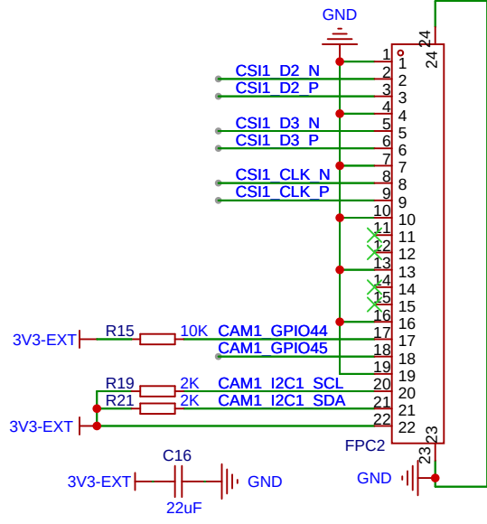
CAMERA1 (CSI1)
